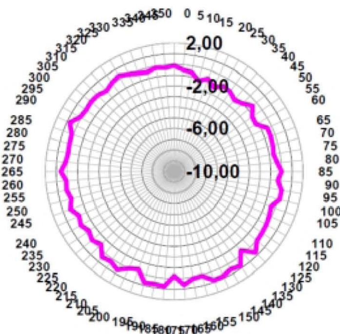
Freq. 1800 MHz H-plane (dBi) V-pol
